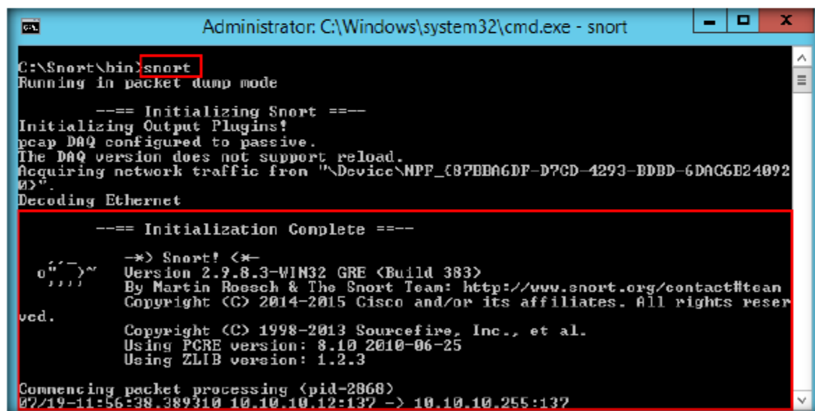
FIGURE 1.5: Basic Snort Command
