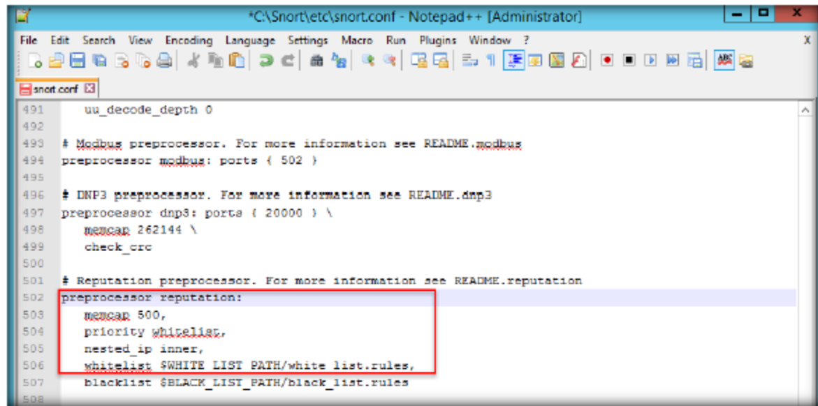
FIGURE 1.17: Configuring Snort.conf File in Notepad++
