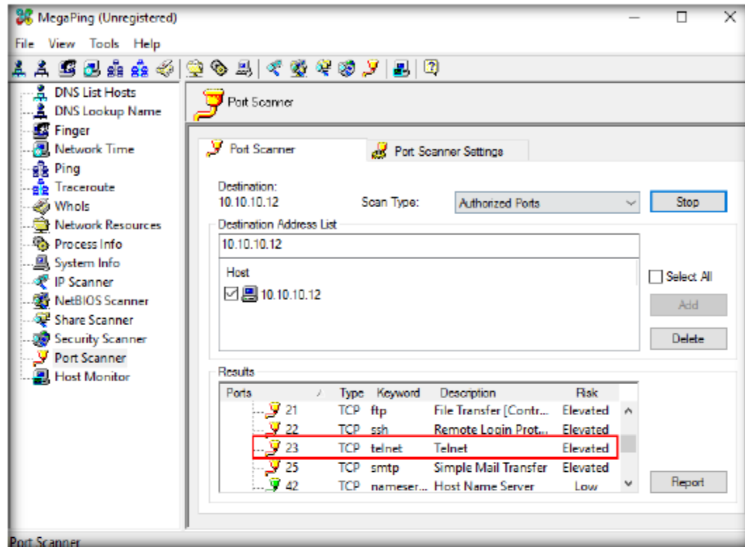
FIGURE 2.13: MegaPing Telnet Port
