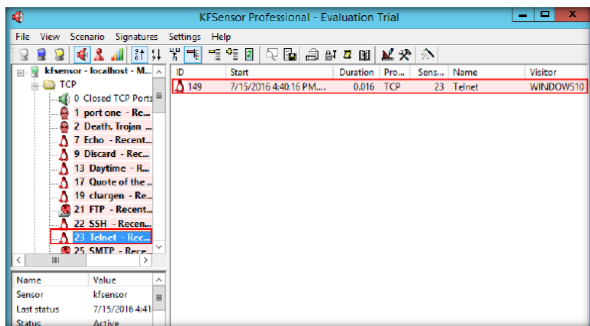
FIGURE 2.14: Telnet port open Alert in KFSensor
