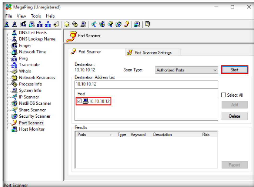
FIGURE 2.12: Beginning the Scan on 10.10.10.12
