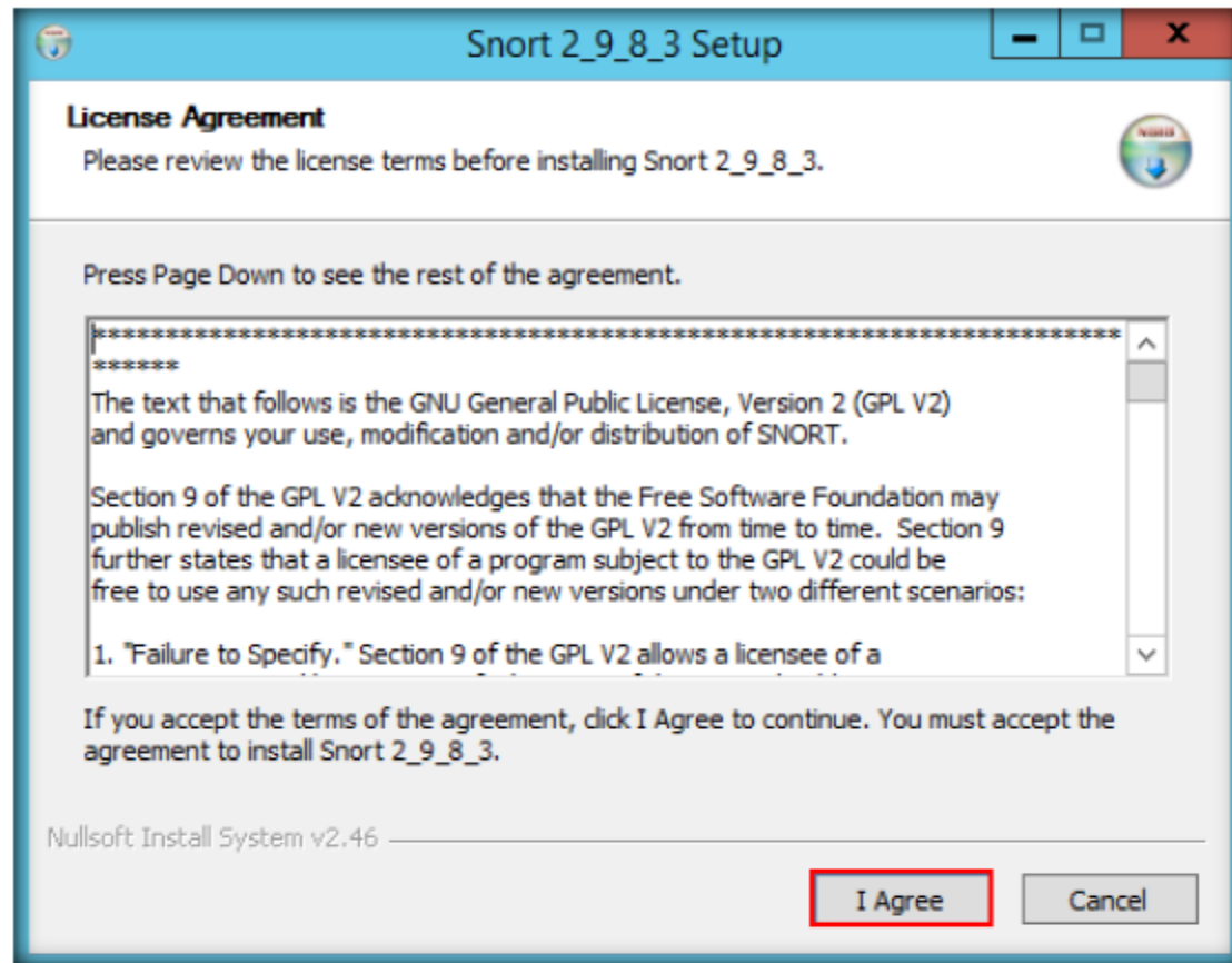
FIGURE 1.1: License Agreement
