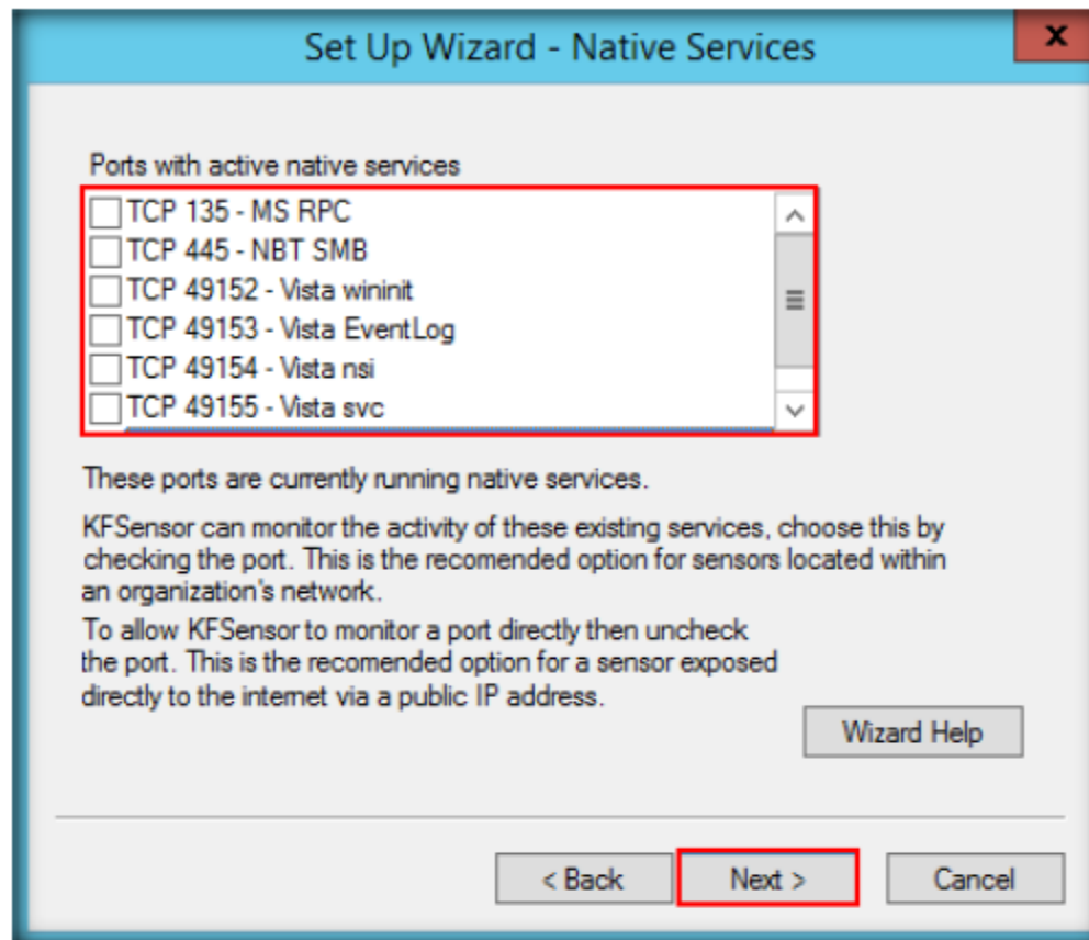
FIGURE 2.3: KFSensor Native Services
