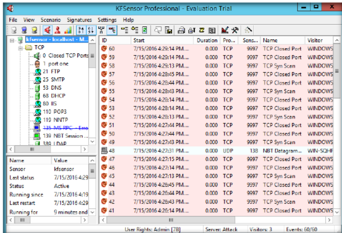
FIGURE 2.6: KFSensor Main Window
