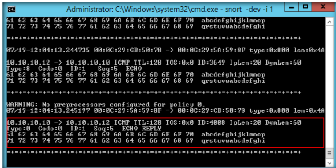
FIGURE 1.9: Snort Showing Captured Ping Request
