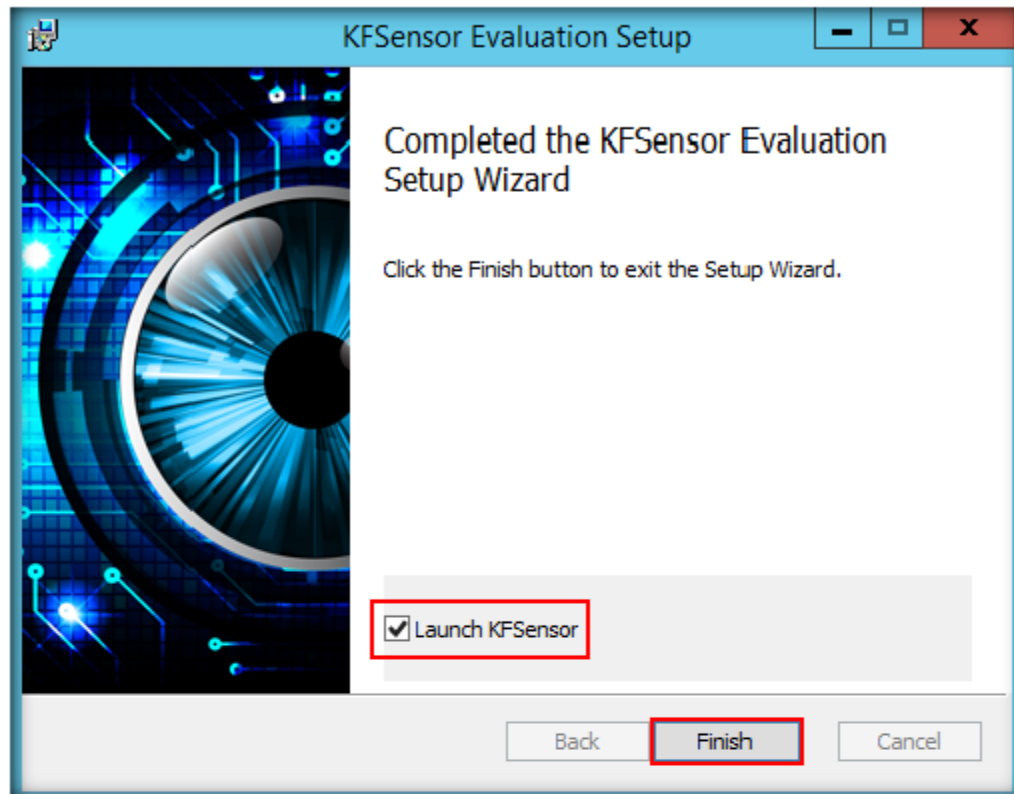
FIGURE 2.1: Launching KFSensor
