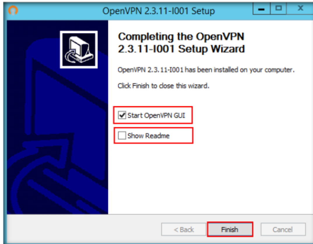
FIGURE 1.3: OpenVPN GUI
